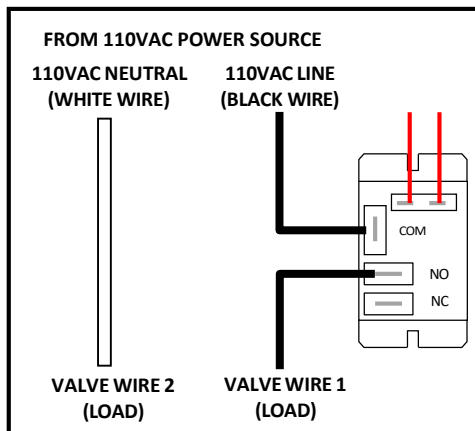
EXAMPLE FOR CONNECTING A 110VAC SOLENOID VALVE
