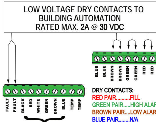
SENSOR PROBE WIRES Front
