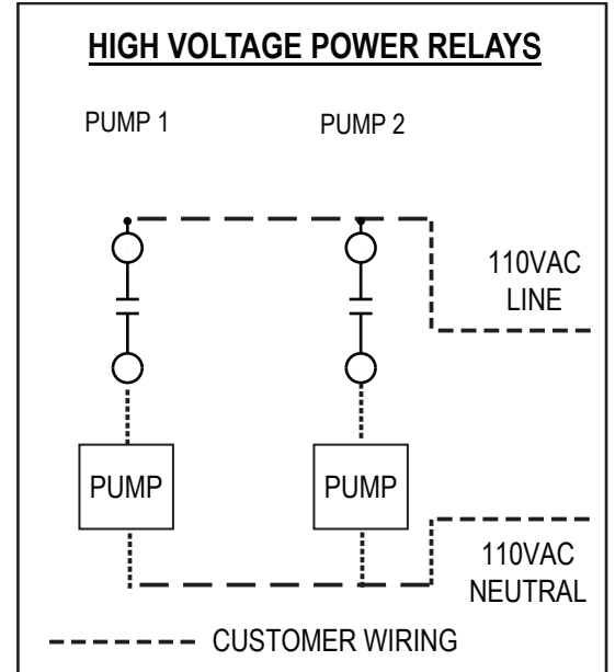
Example of 100VAC devices wired to power relays
